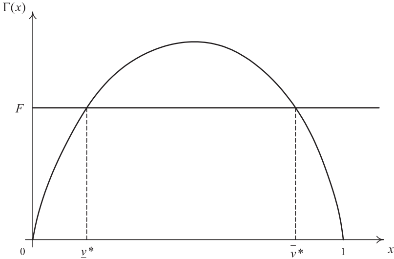
Fig. 1. Entry cut-off equilibria.
