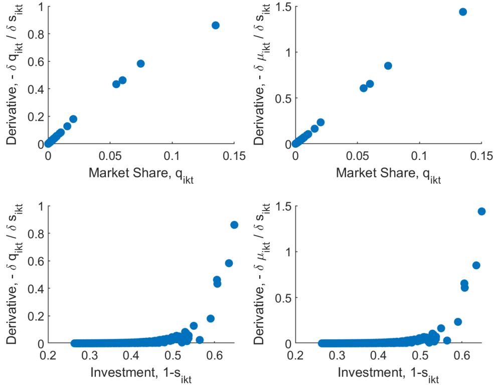
Figure 25: Partial Derivatives
